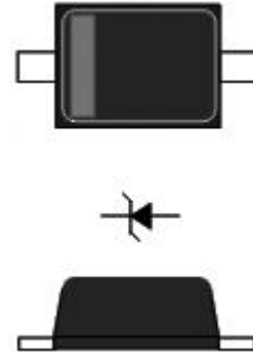
SOD-523
