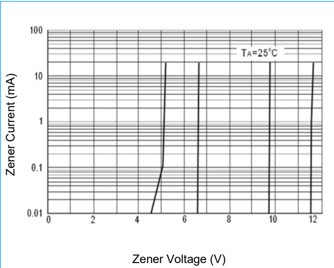
Fig1. Zener Breakdown Characteristic
