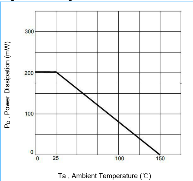
Fig7. Power Derating Curve
